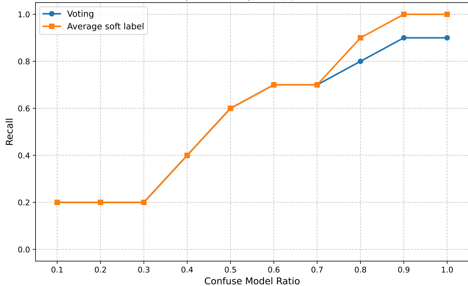
Recall | Round 10 | Entropy Ratio 0.30
