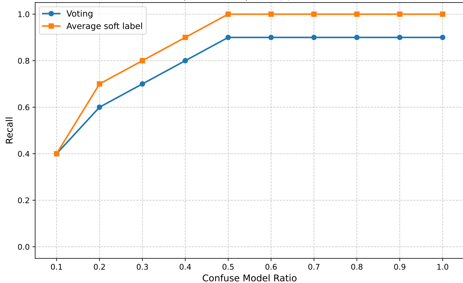
Recall | Round 10 | Entropy Ratio 0.50
