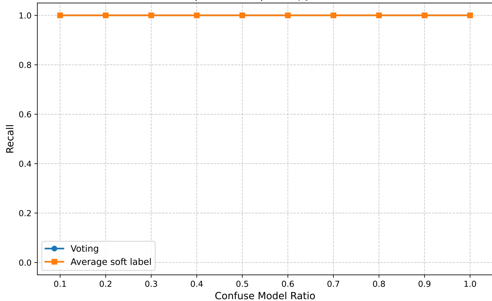
Recall | Round 10 | Entropy Ratio 0.90
