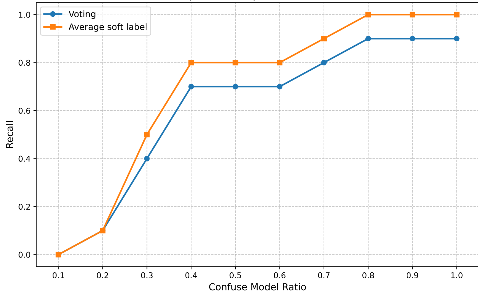
Recall | Round 15 | Entropy Ratio 0.35
