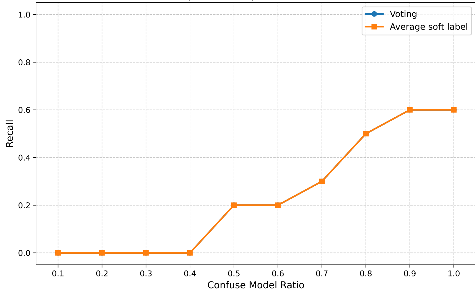
Recall | Round 20 | Entropy Ratio 0.15
