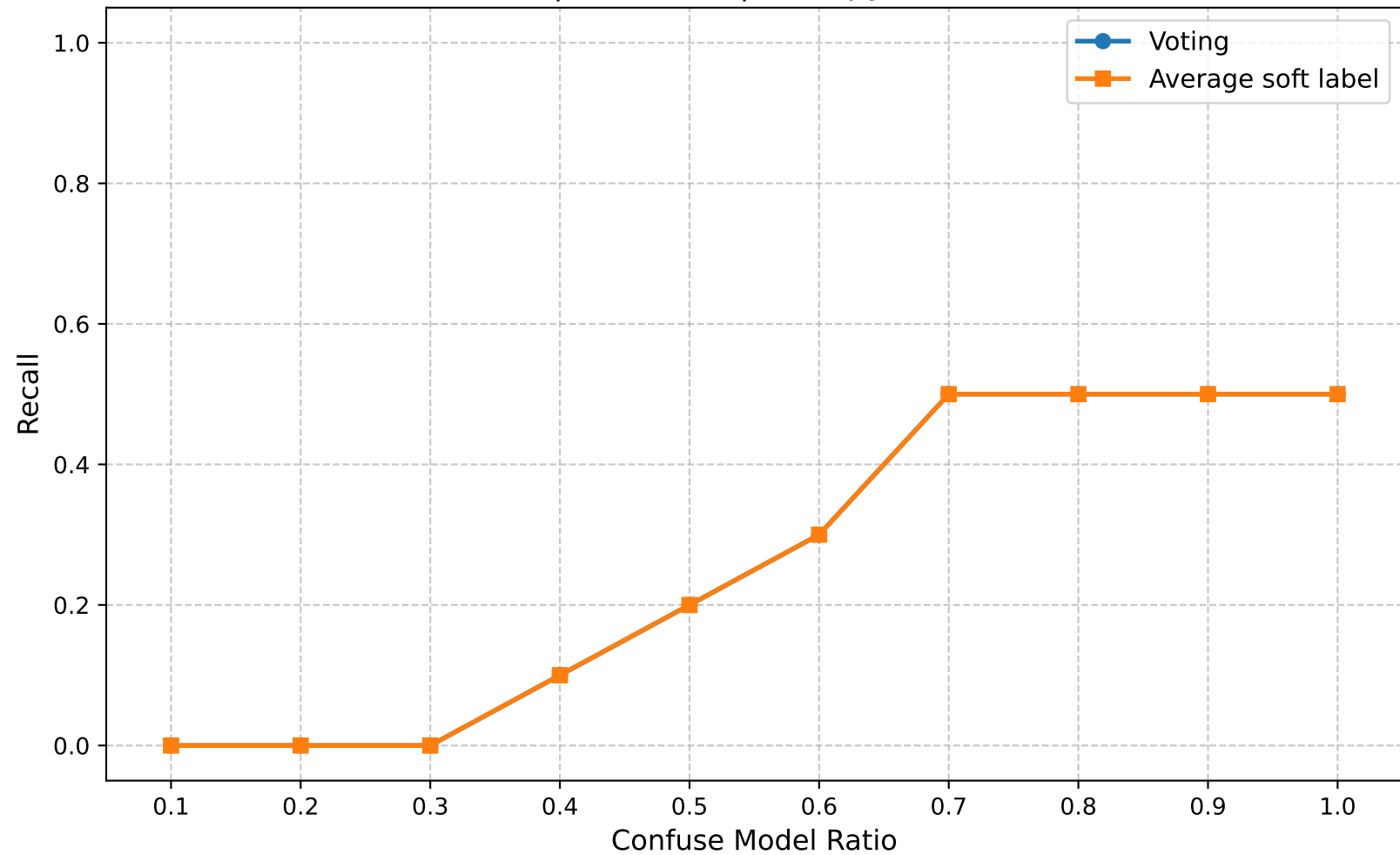
Recall | Round 25 | Entropy Ratio 0.15
