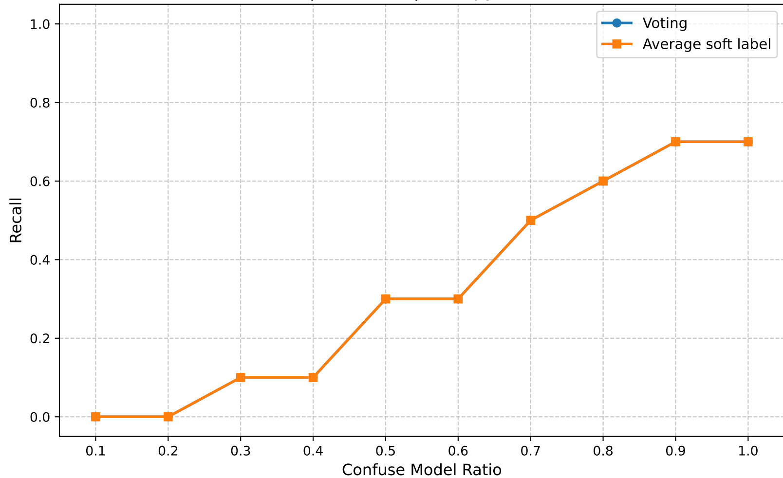
Recall | Round 25 | Entropy Ratio 0.20
