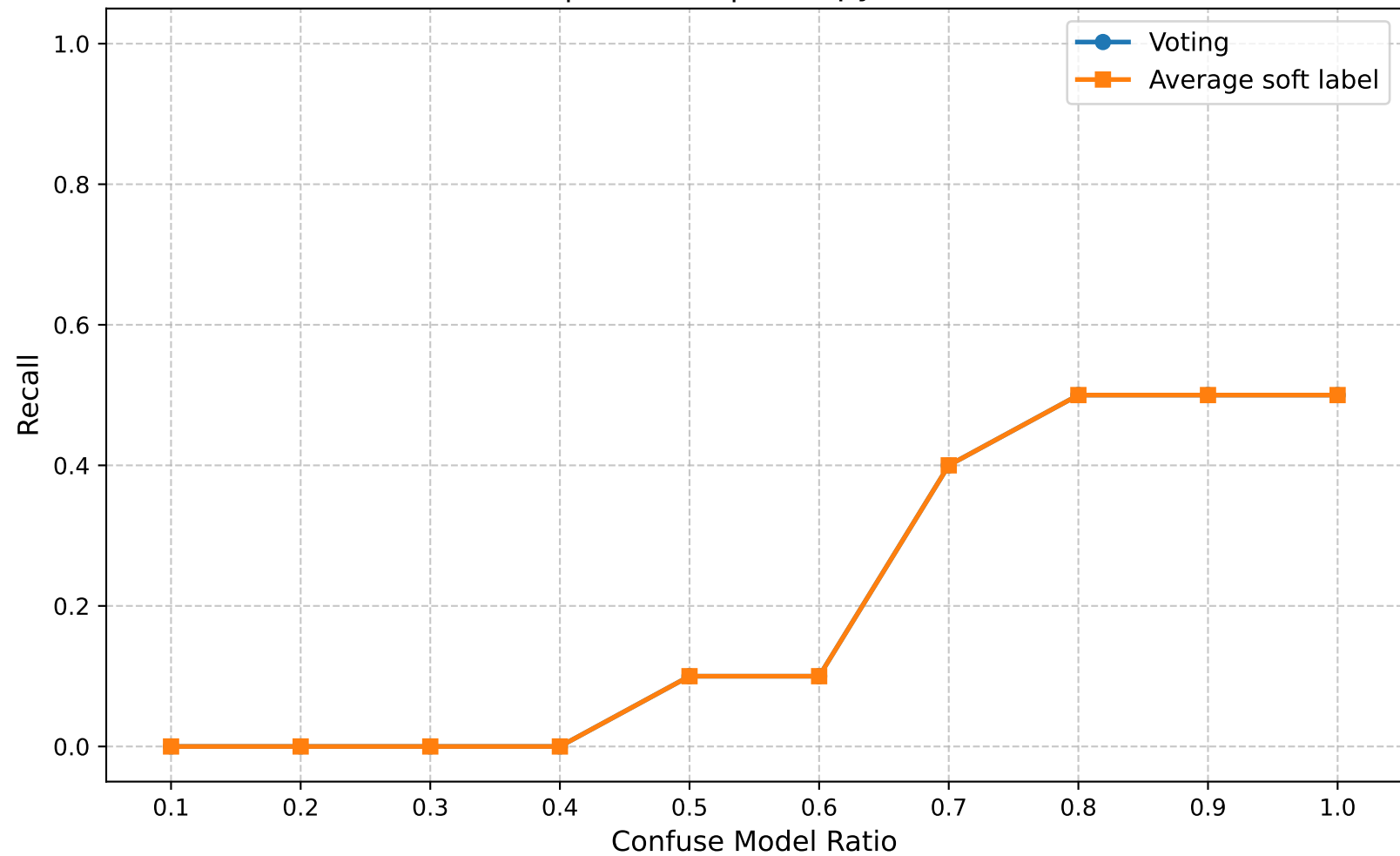
Recall | Round 5 | Entropy Ratio 0.10
