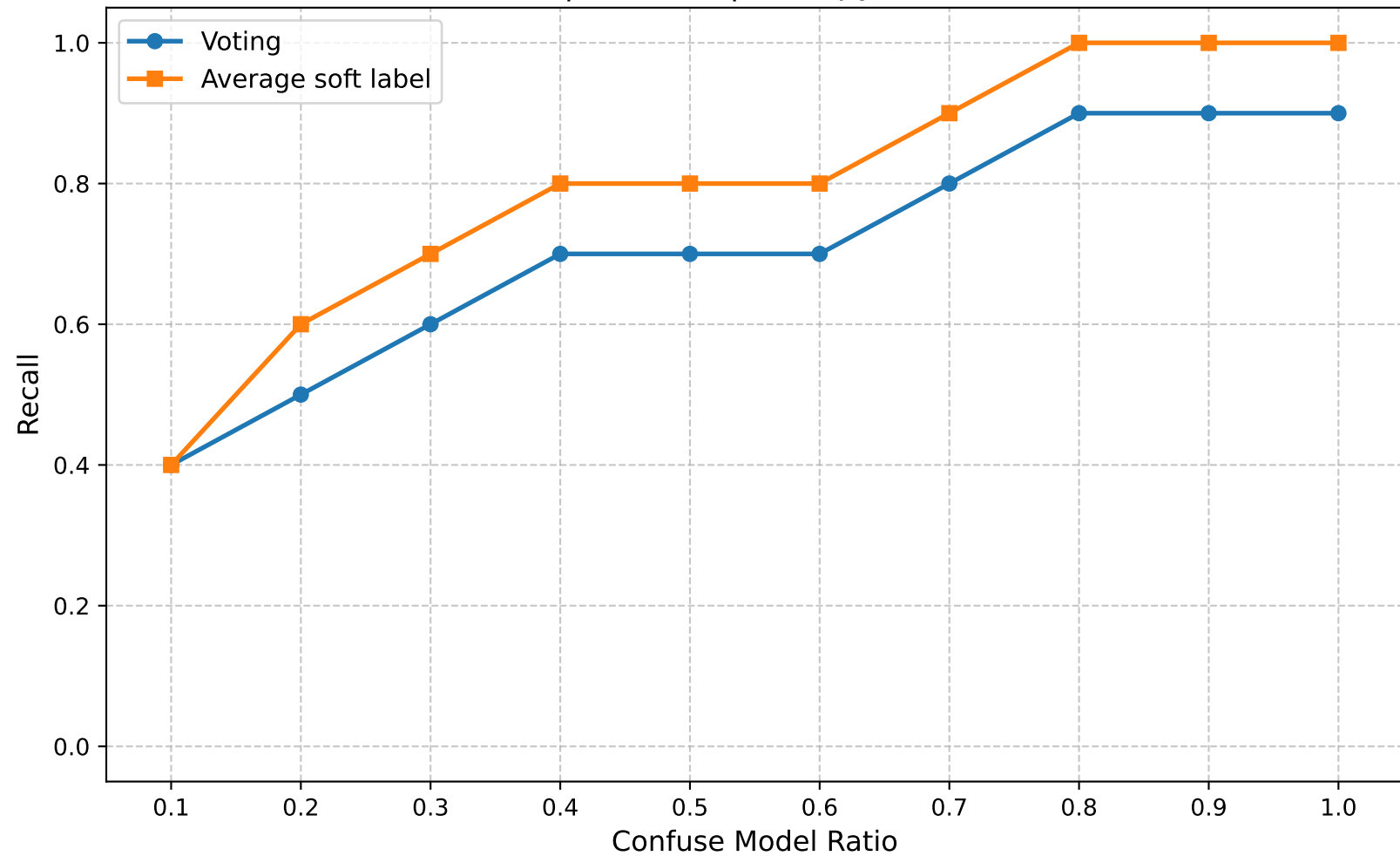
Recall | Round 5 | Entropy Ratio 0.35
