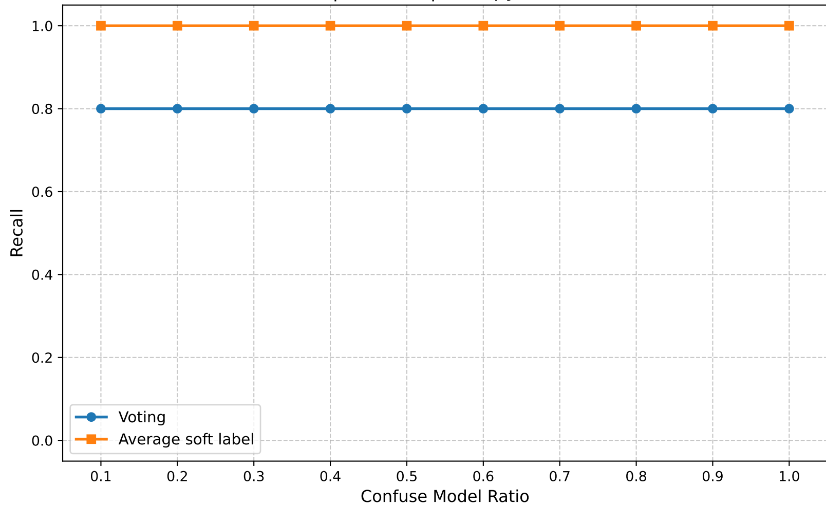
Recall | Round 5 | Entropy Ratio 0.85
