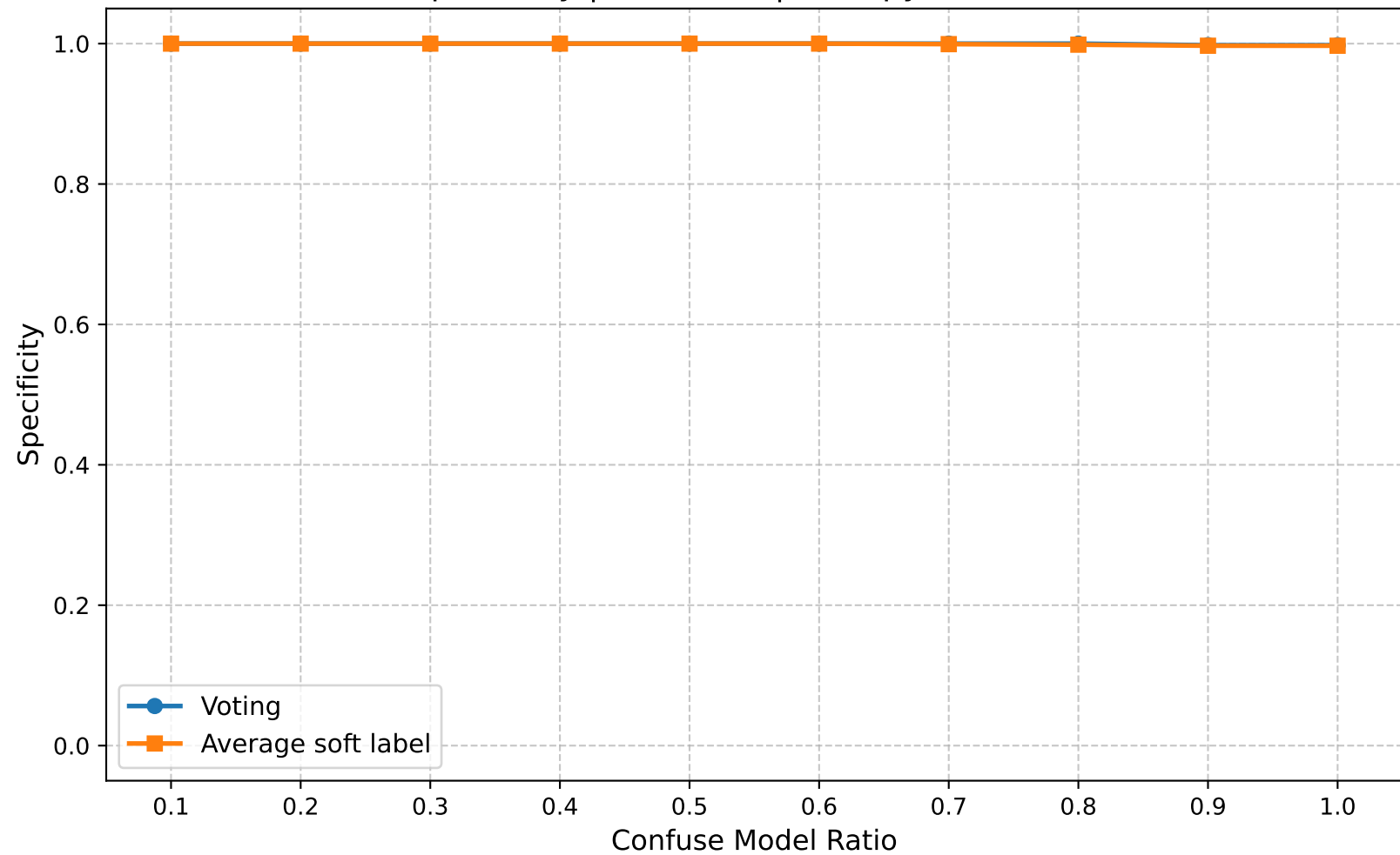
Specificity | Round 10 | Entropy Ratio 0.15
