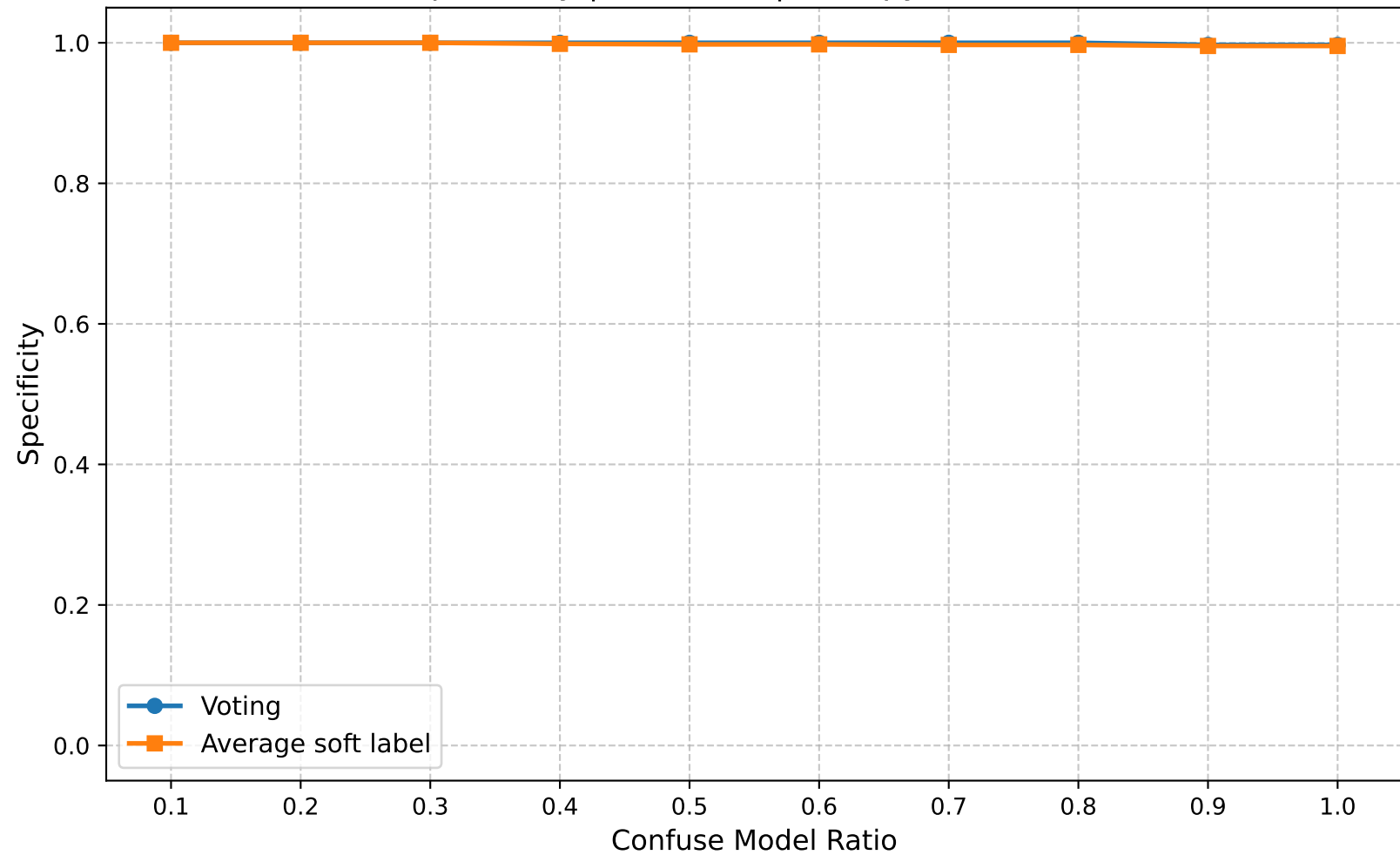
Specificity | Round 10 | Entropy Ratio 0.60
