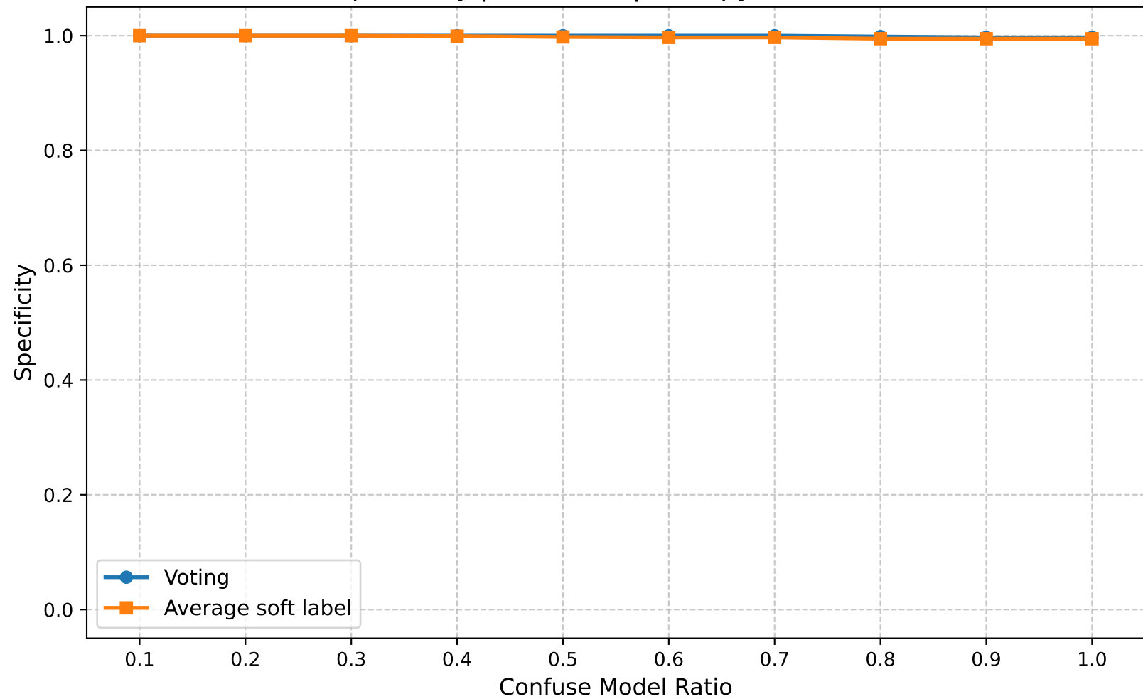
Specificity | Round 20 | Entropy Ratio 0.65
