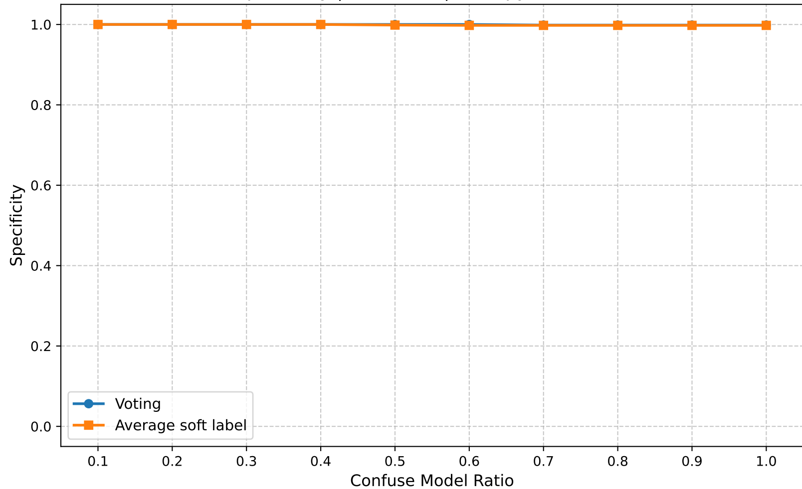
Specificity | Round 25 | Entropy Ratio 0.50
