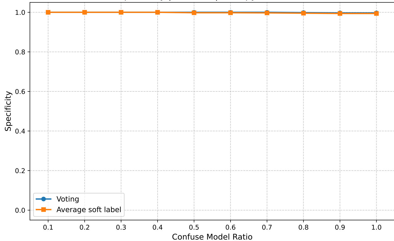
Specificity | Round 5 | Entropy Ratio 0.60
