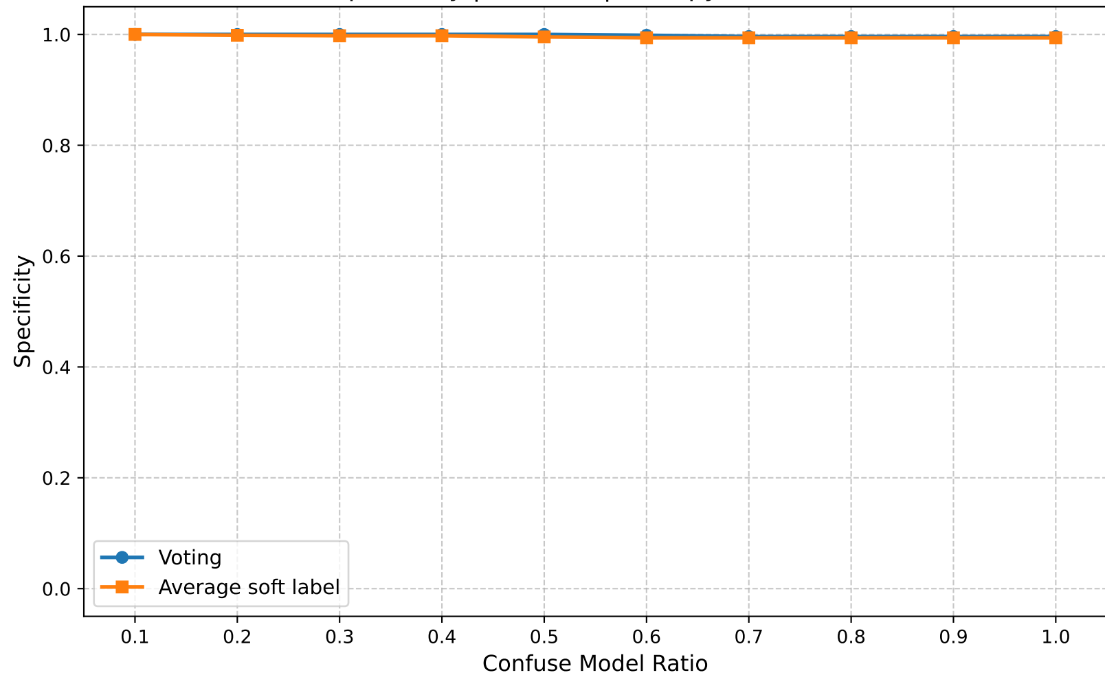
Specificity | Round 5 | Entropy Ratio 0.80
