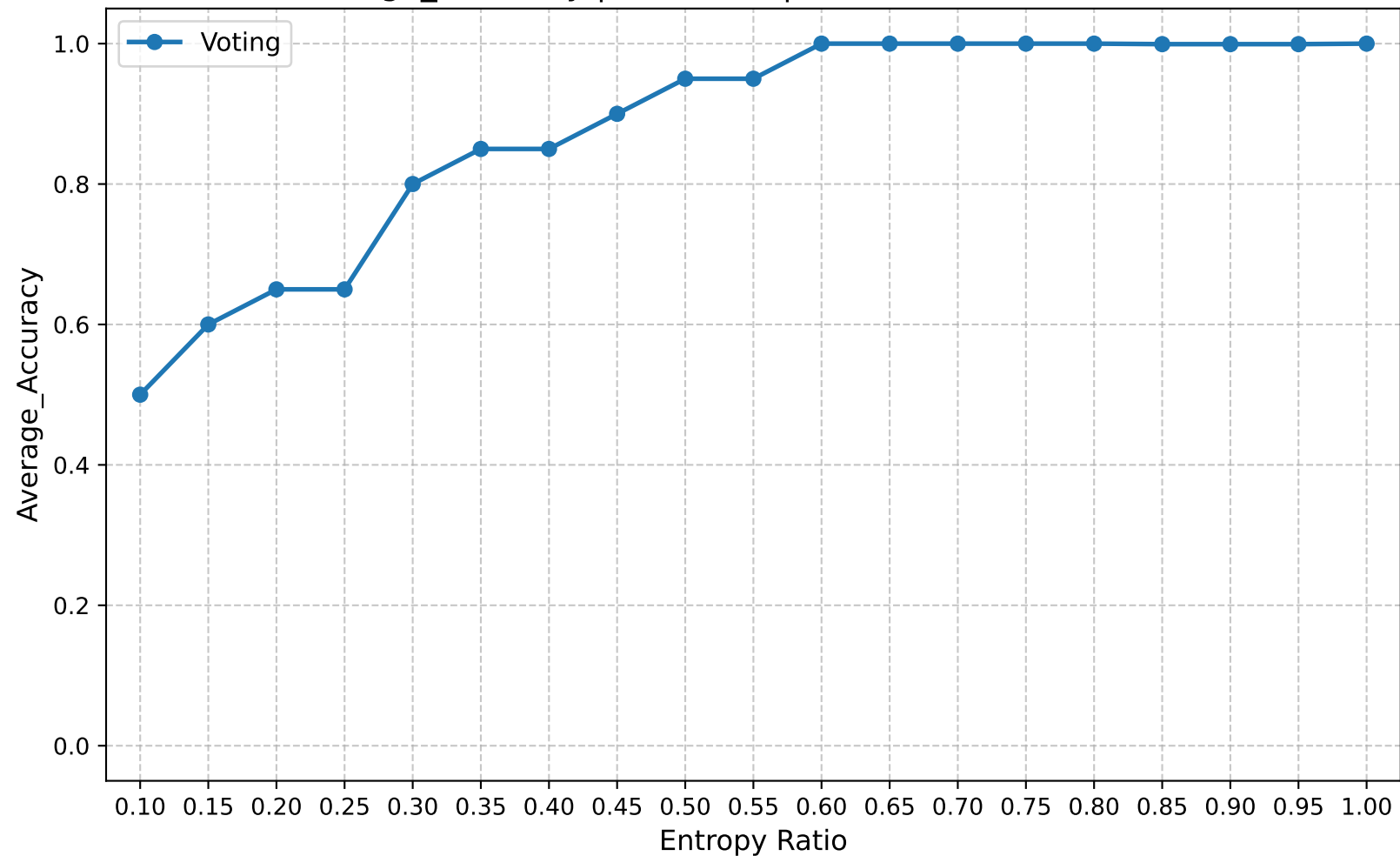
Average_Accuracy | Round 10 | Confuse Model Ratio 0.50
