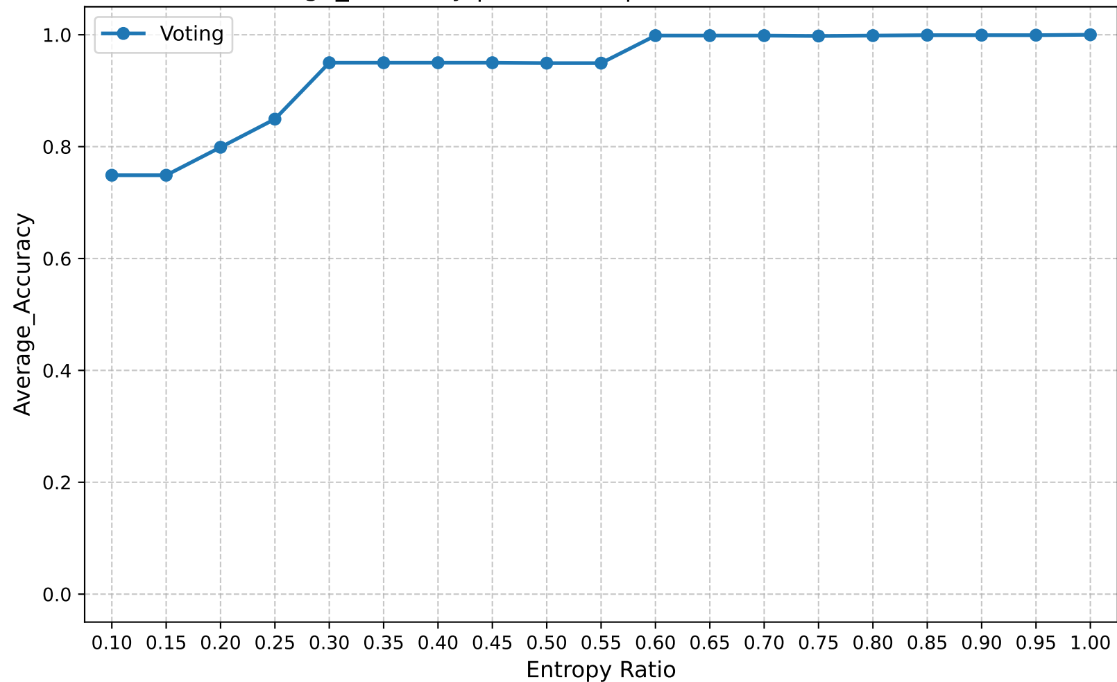
Average_Accuracy | Round 10 | Confuse Model Ratio 1.00
