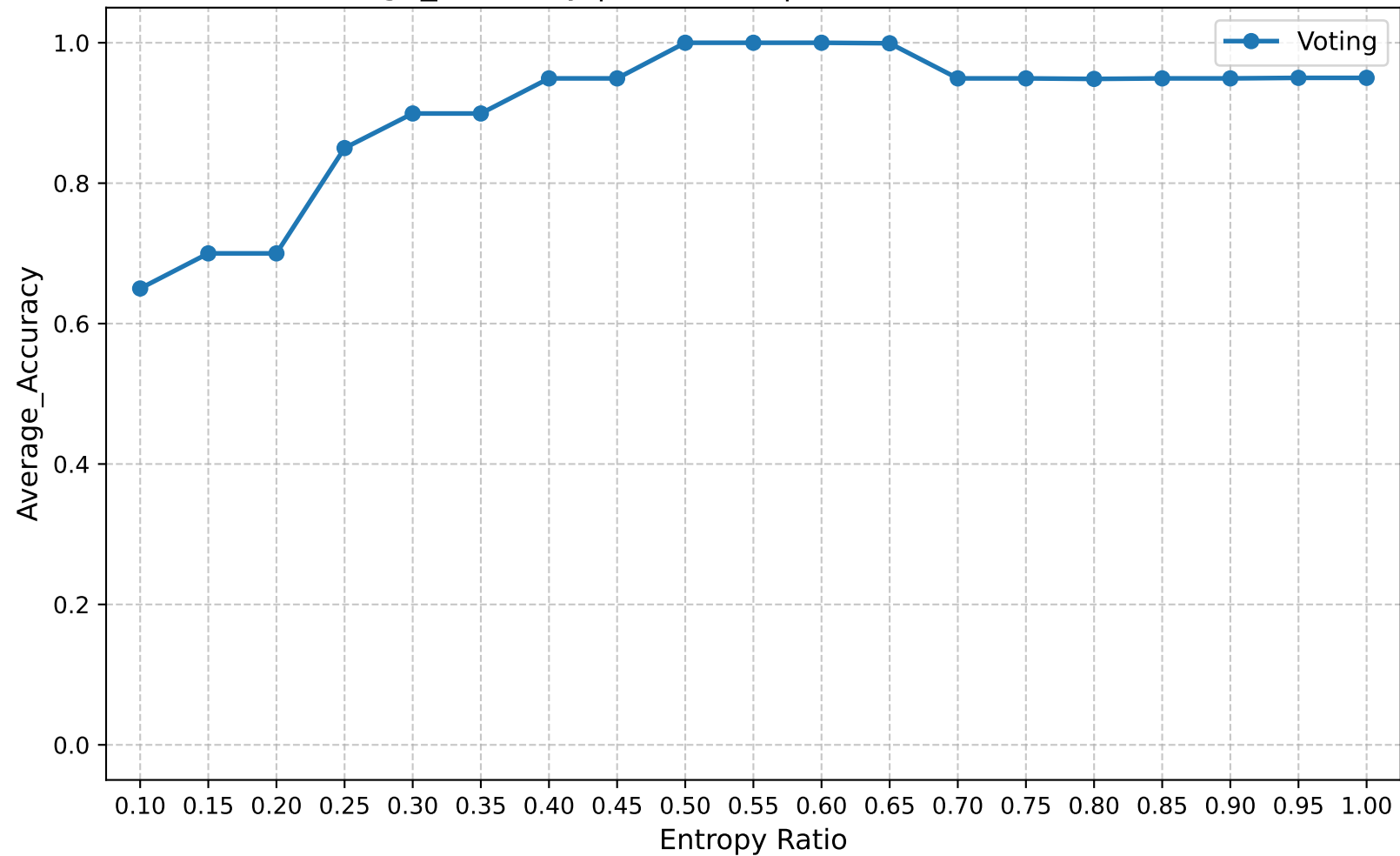
Average_Accuracy | Round 15 | Confuse Model Ratio 0.70
