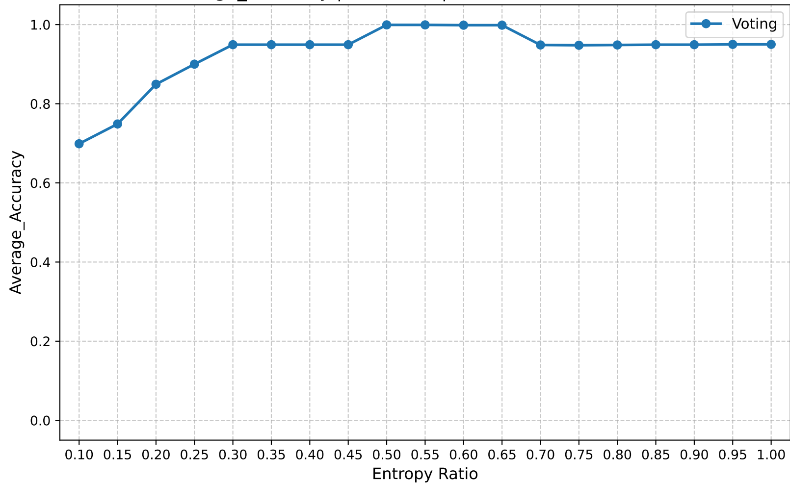
Average_Accuracy | Round 15 | Confuse Model Ratio 1.00
