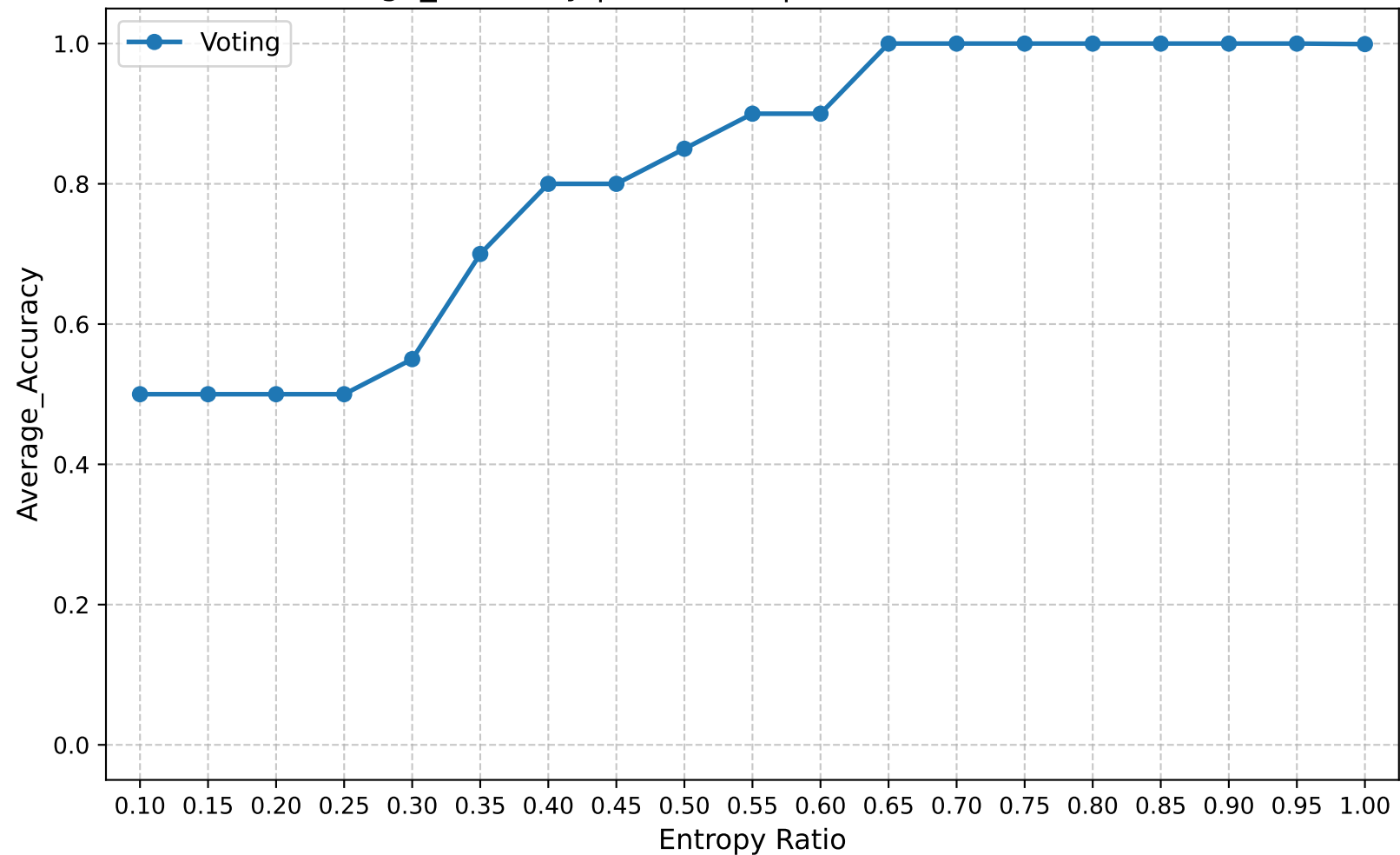
Average_Accuracy | Round 25 | Confuse Model Ratio 0.20
