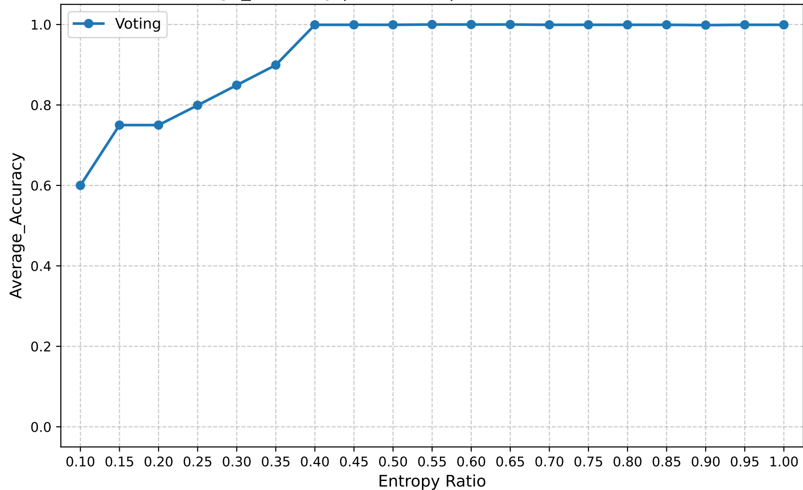
Average_Accuracy | Round 25 | Confuse Model Ratio 0.70
