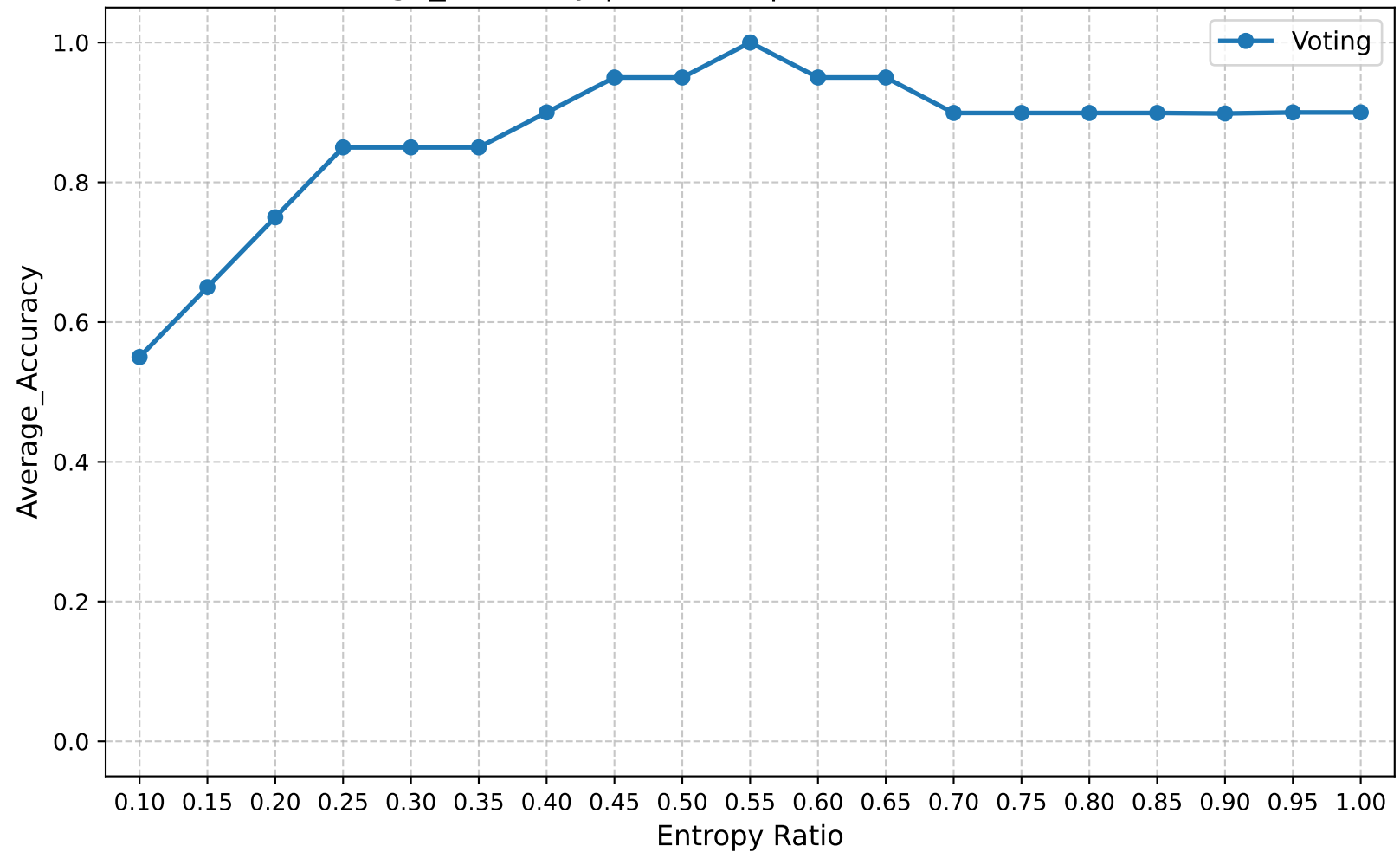
Average_Accuracy | Round 5 | Confuse Model Ratio 0.60
