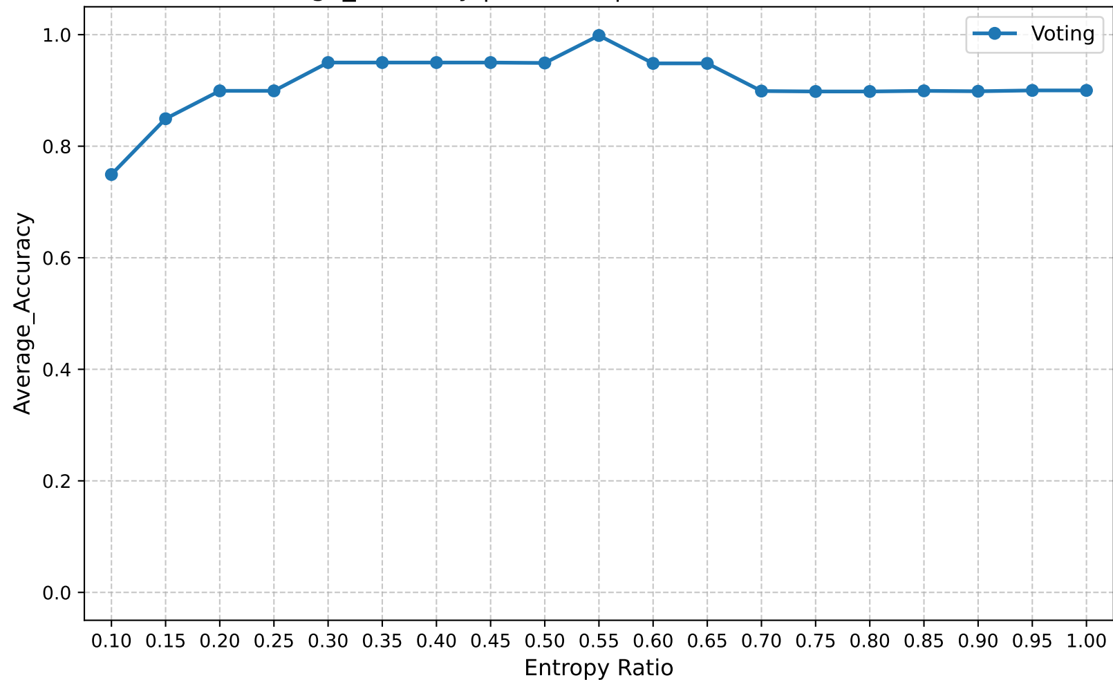
Average_Accuracy | Round 5 | Confuse Model Ratio 0.90
