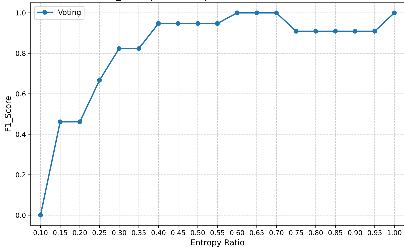
F1_Score | Round 10 | Confuse Model Ratio 0.60
