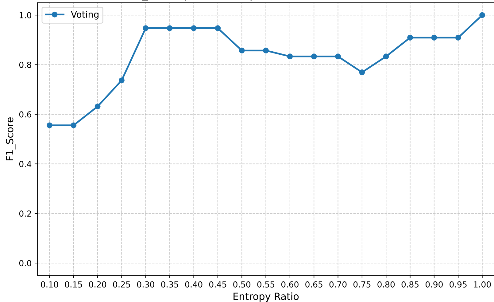
F1_Score | Round 10 | Confuse Model Ratio 0.90
