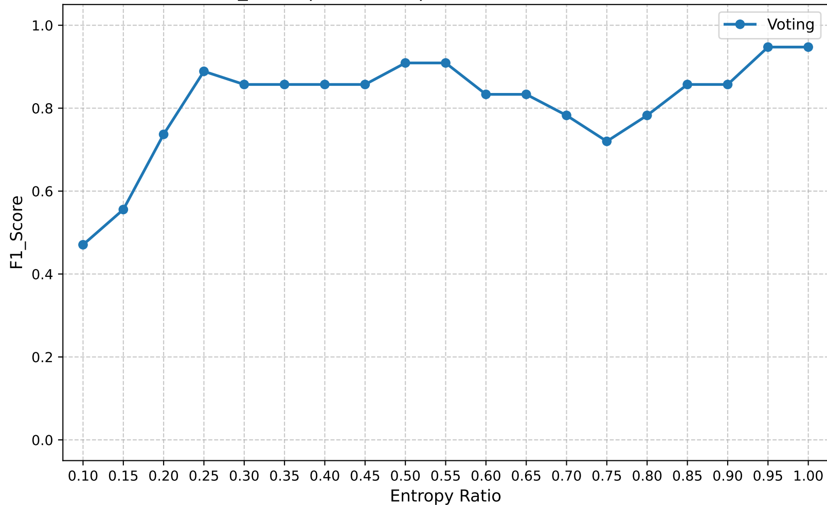
F1_Score | Round 15 | Confuse Model Ratio 1.00
