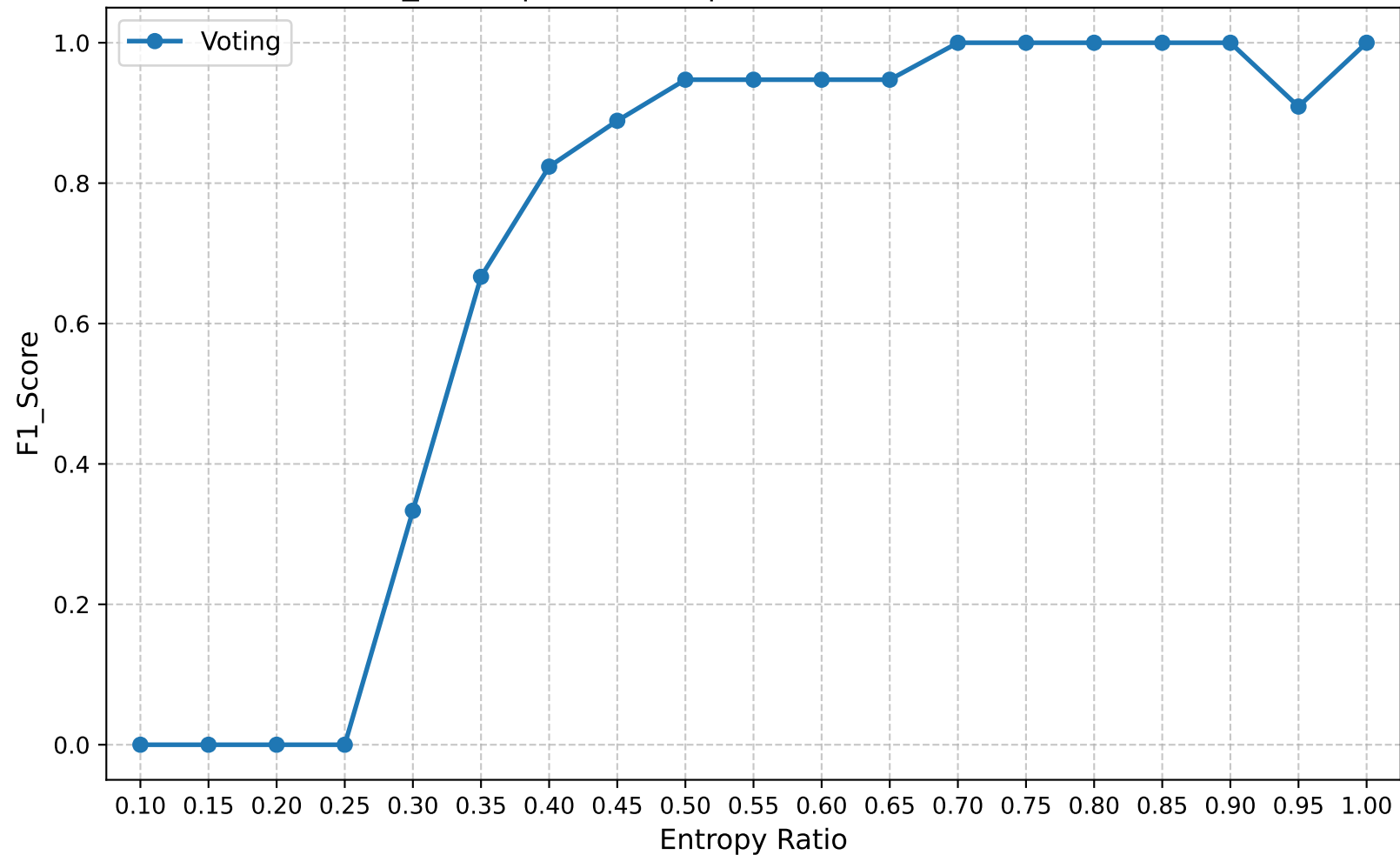
F1_Score | Round 20 | Confuse Model Ratio 0.30
