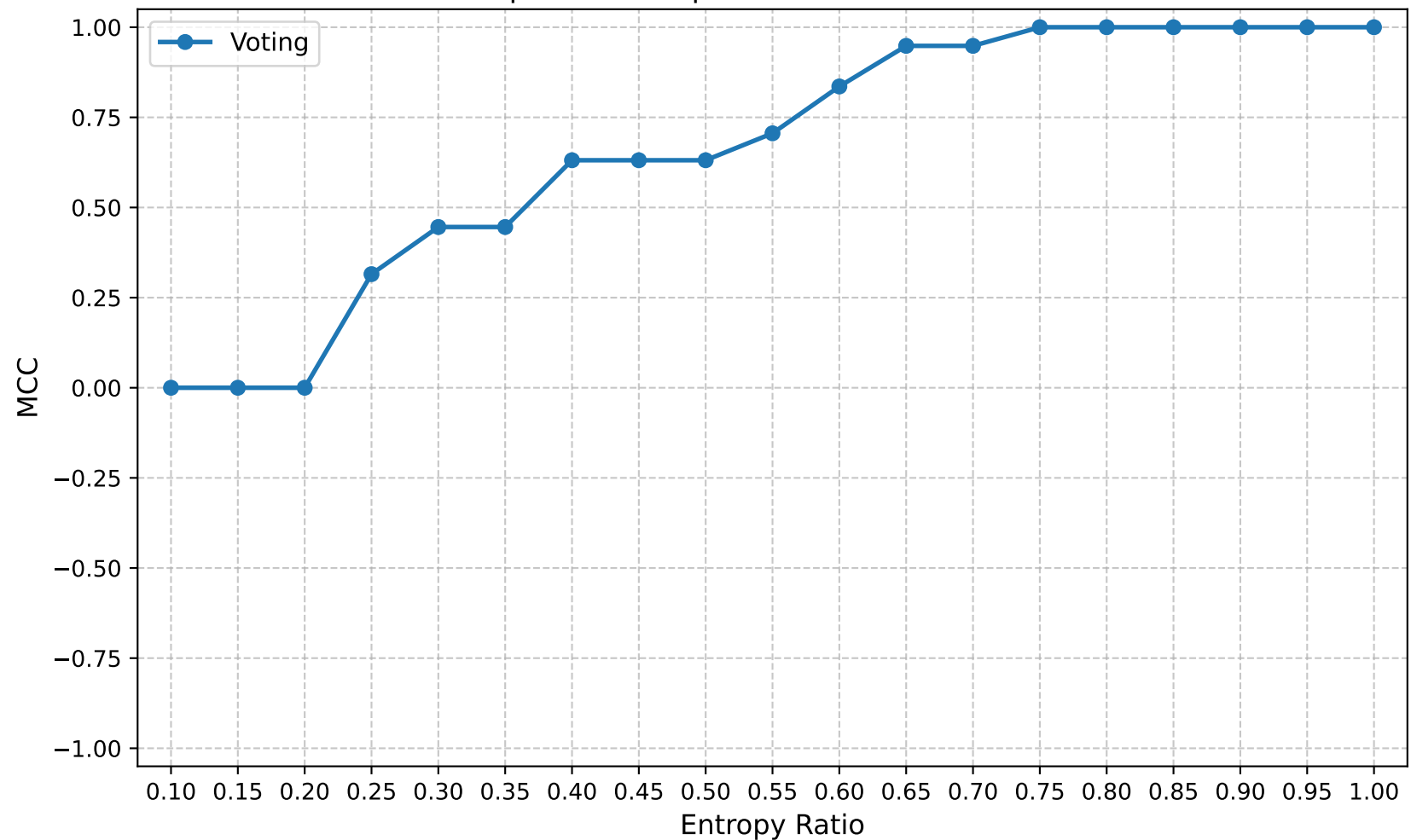
MCC | Round 10 | Confuse Model Ratio 0.10
