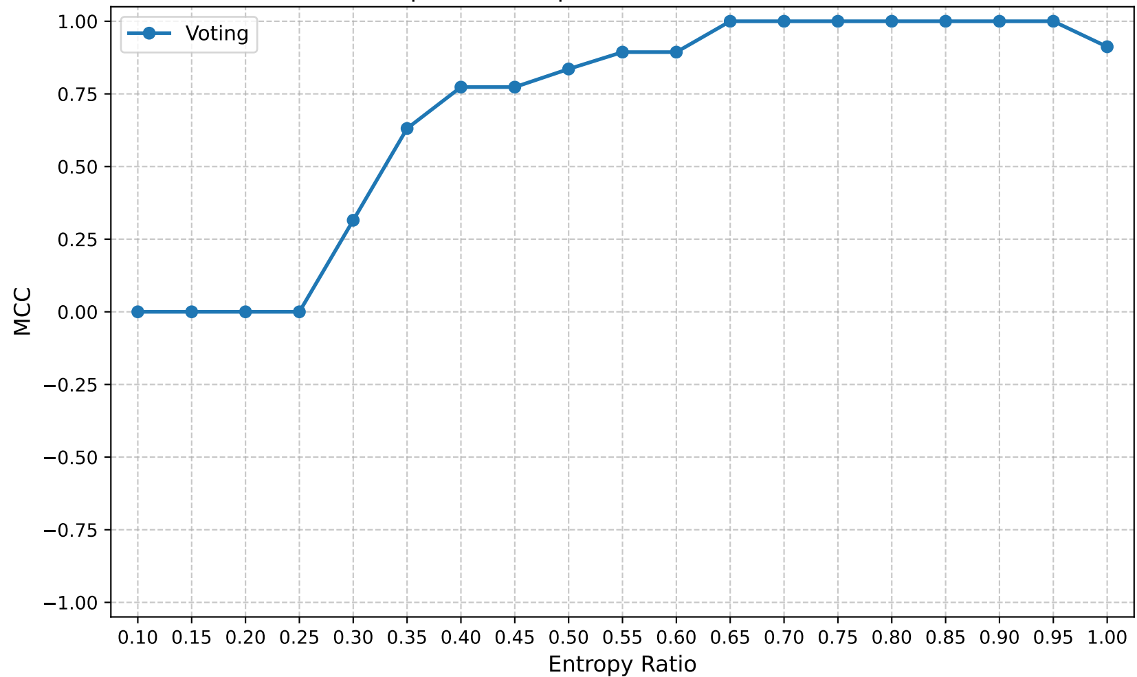
MCC | Round 25 | Confuse Model Ratio 0.20
