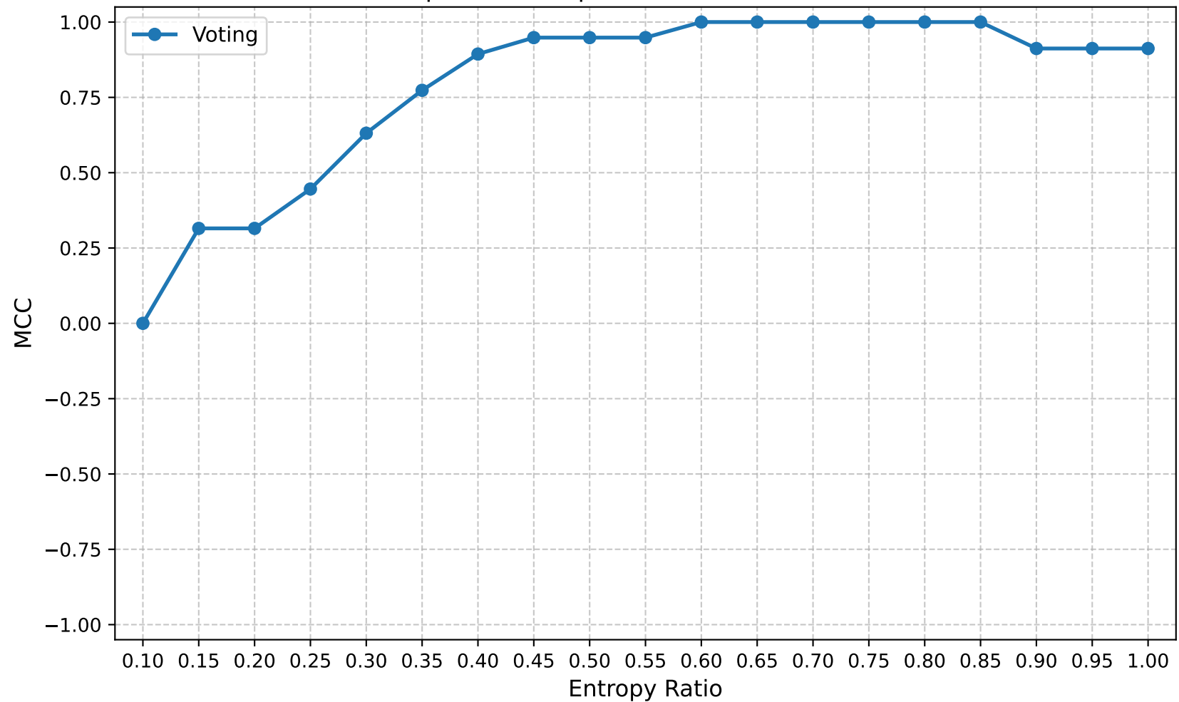
MCC | Round 25 | Confuse Model Ratio 0.40
