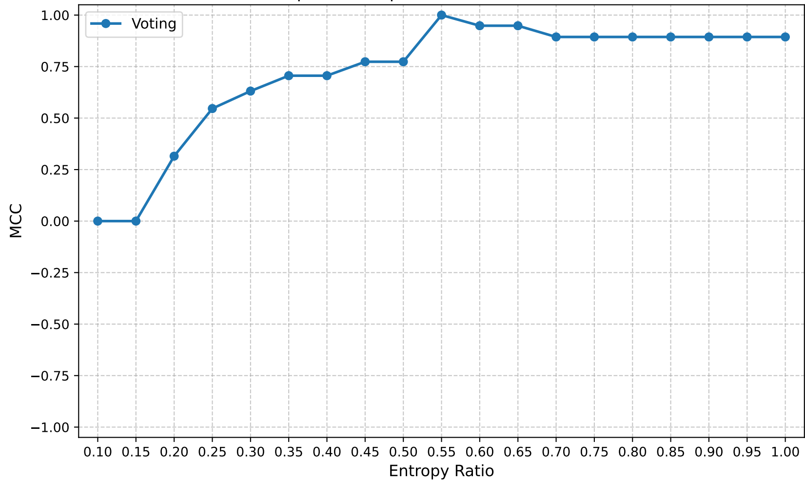
MCC | Round 5 | Confuse Model Ratio 0.20
