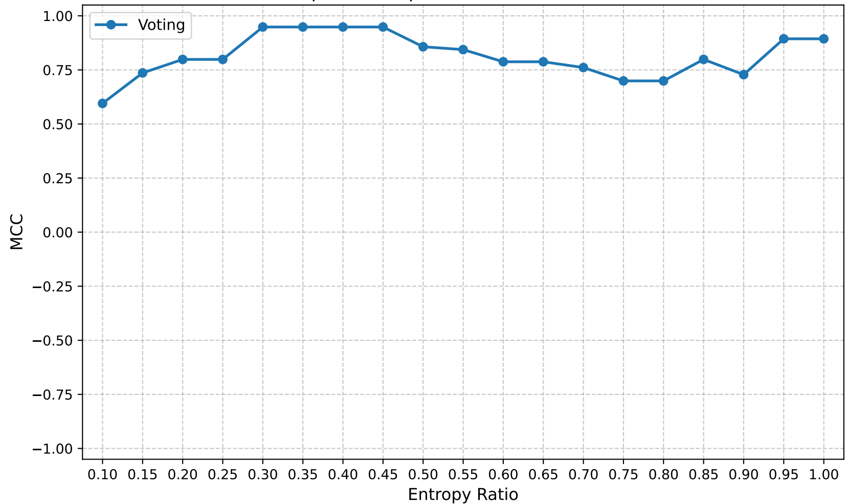
MCC | Round 5 | Confuse Model Ratio 0.90
