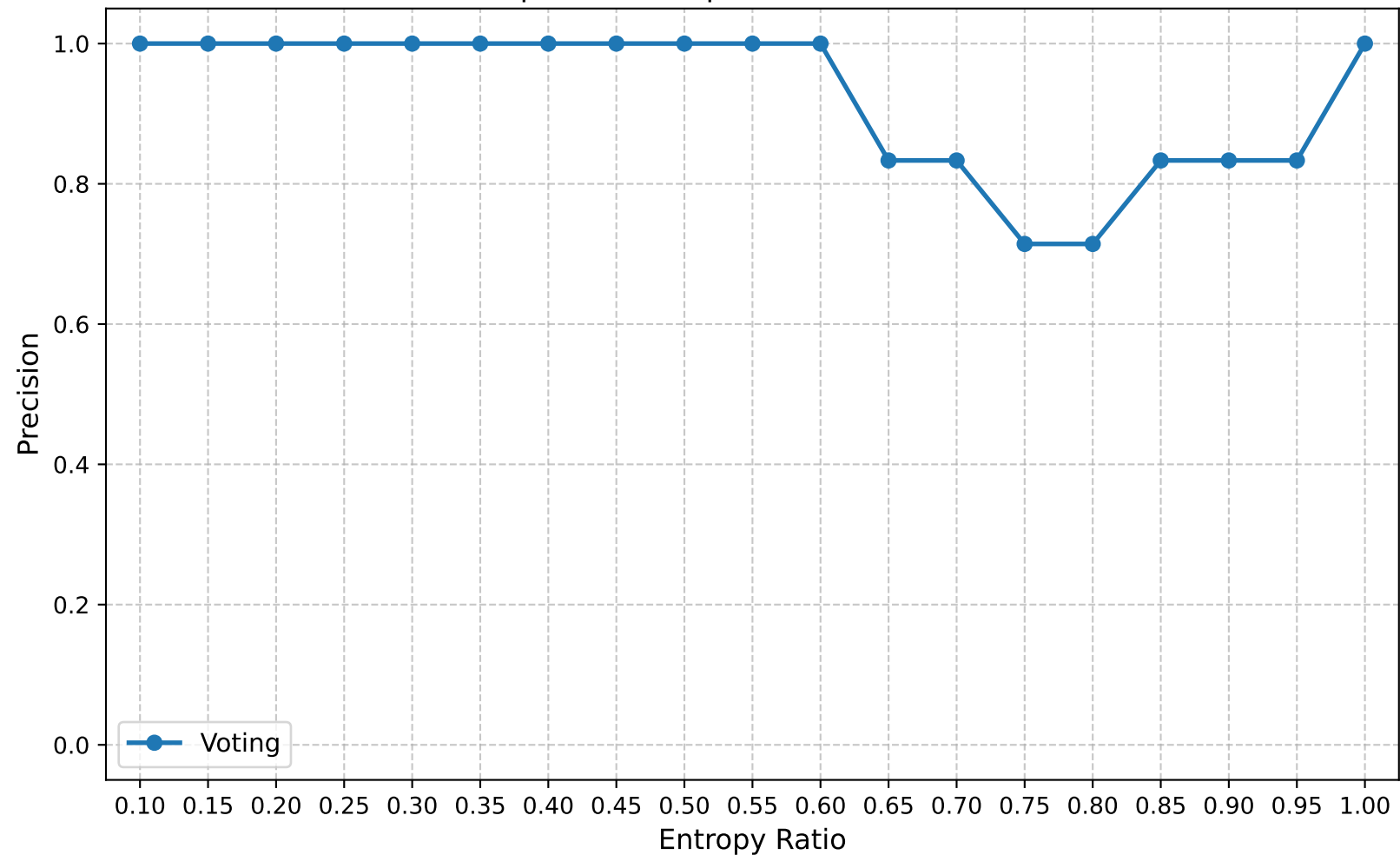
Precision | Round 10 | Confuse Model Ratio 0.80
