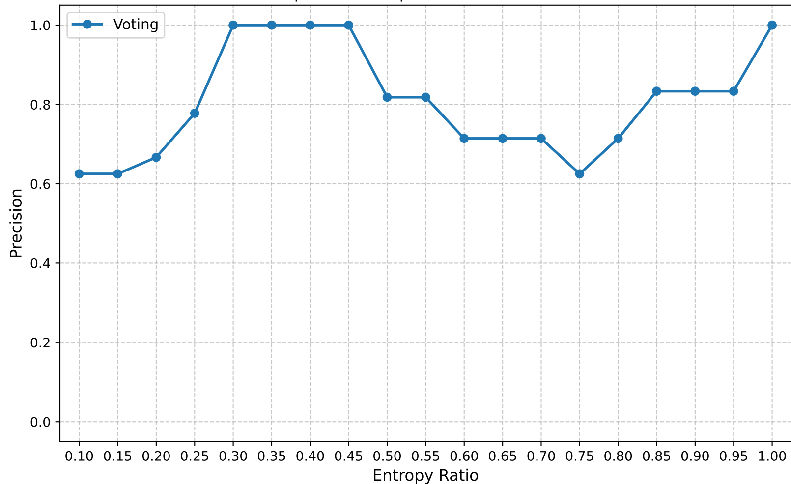
Precision | Round 10 | Confuse Model Ratio 1.00
