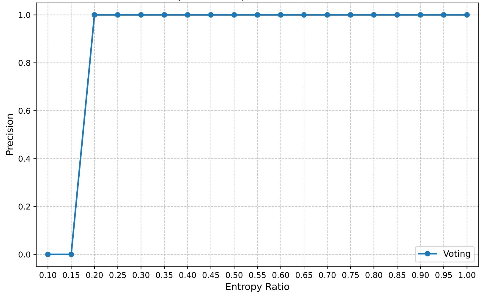
Precision | Round 15 | Confuse Model Ratio 0.40
