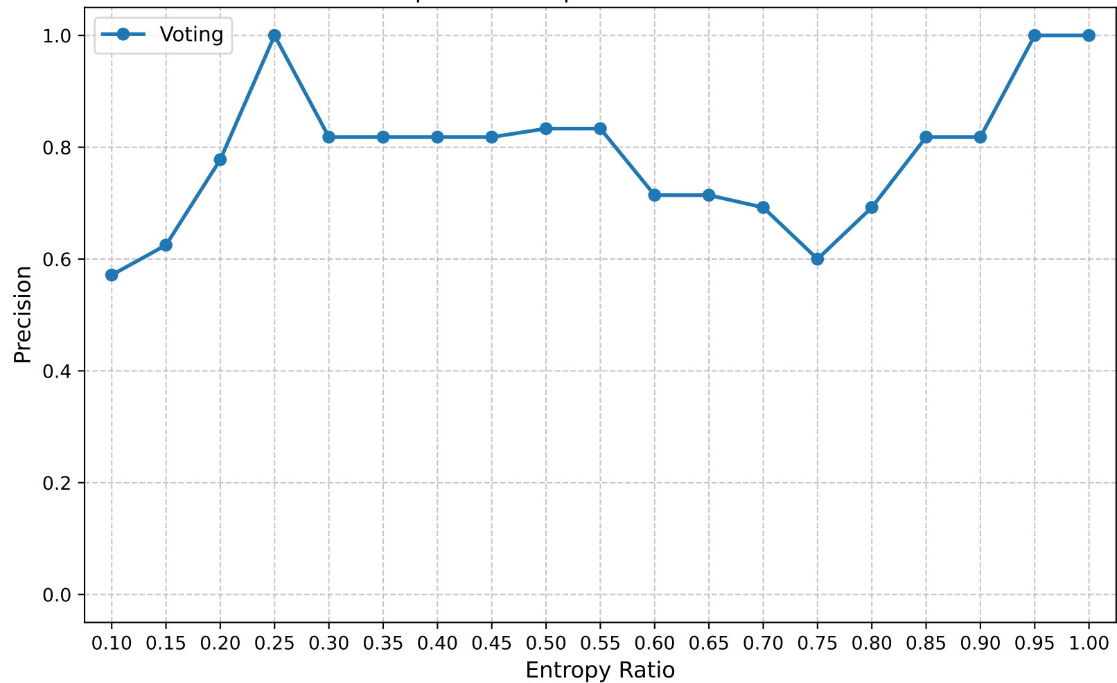
Precision | Round 15 | Confuse Model Ratio 1.00
