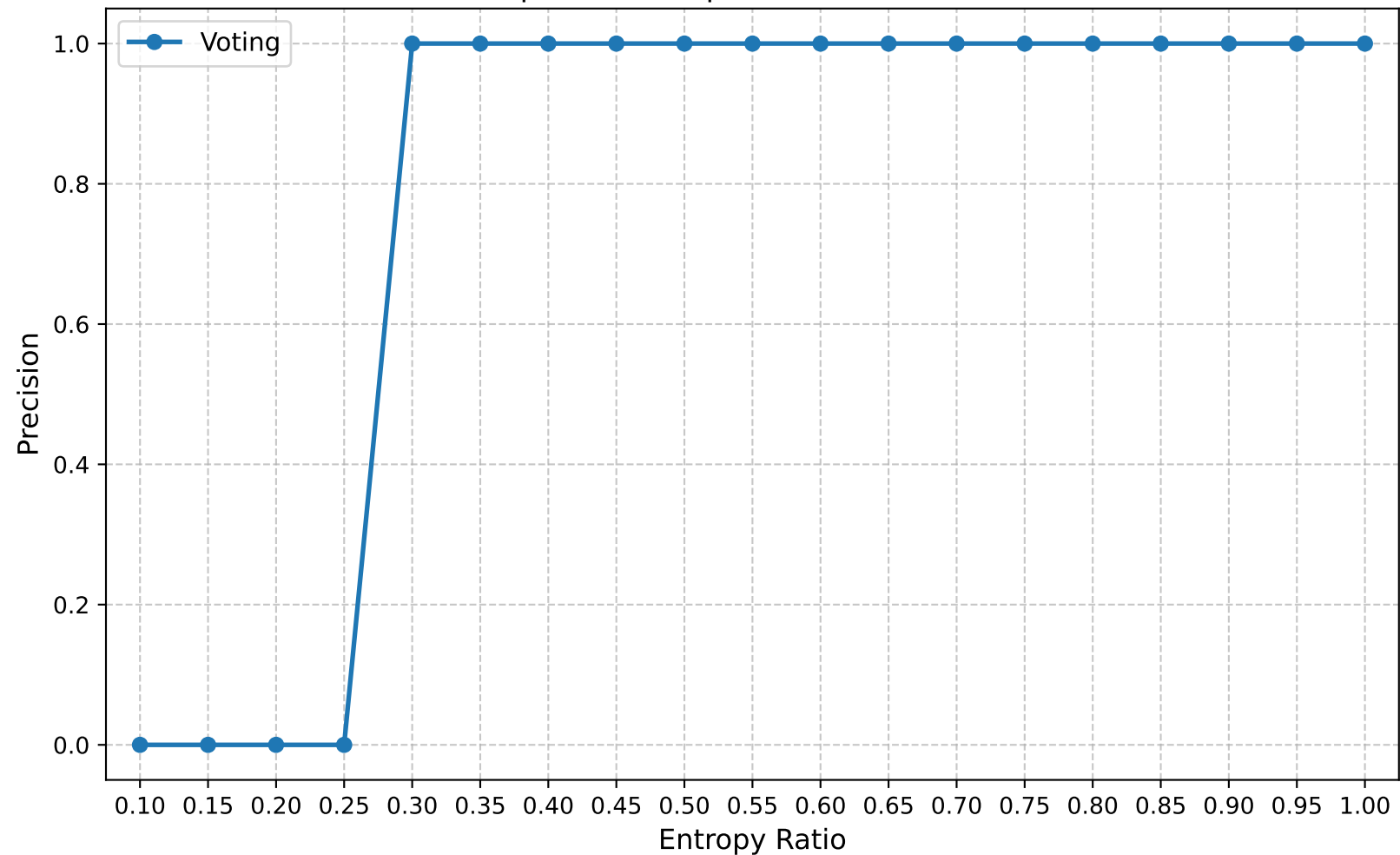
Precision | Round 20 | Confuse Model Ratio 0.20
