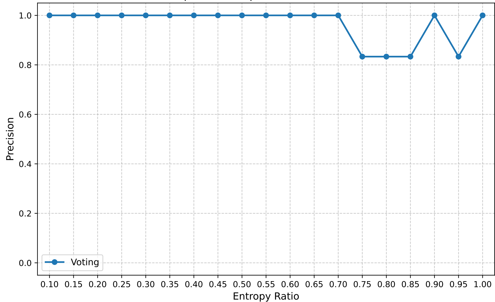
Precision | Round 20 | Confuse Model Ratio 0.60
