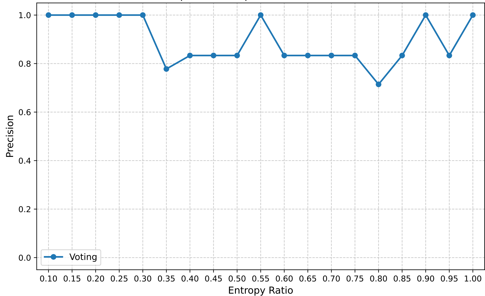
Precision | Round 20 | Confuse Model Ratio 0.80
