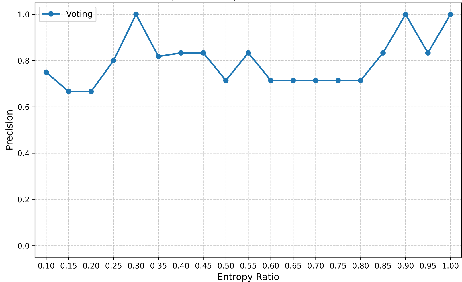
Precision | Round 20 | Confuse Model Ratio 1.00
