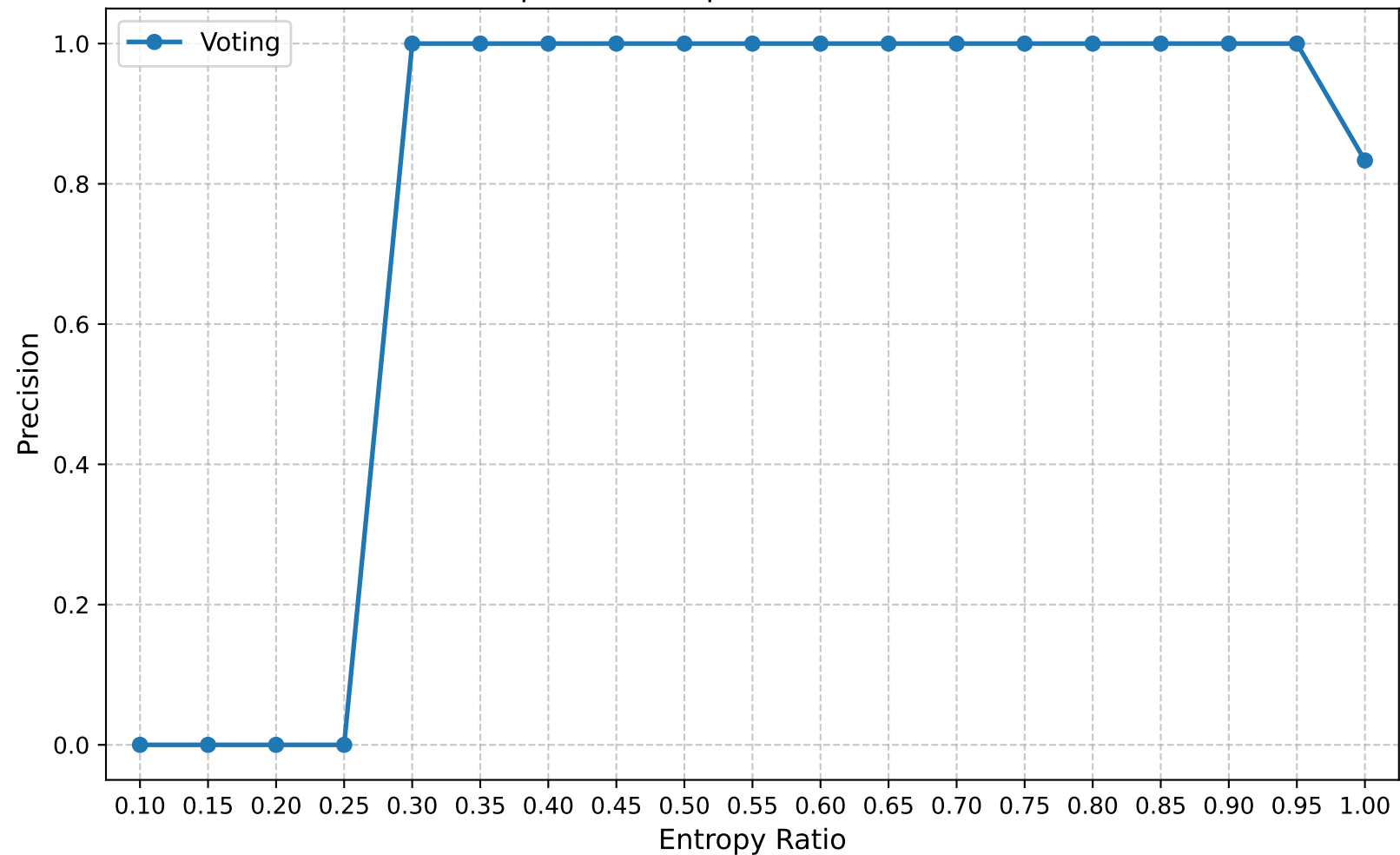
Precision | Round 25 | Confuse Model Ratio 0.10
