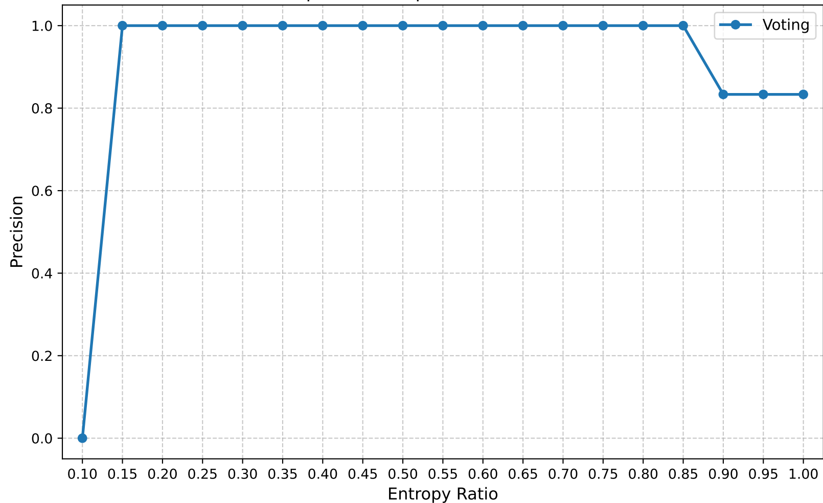
Precision | Round 25 | Confuse Model Ratio 0.40
