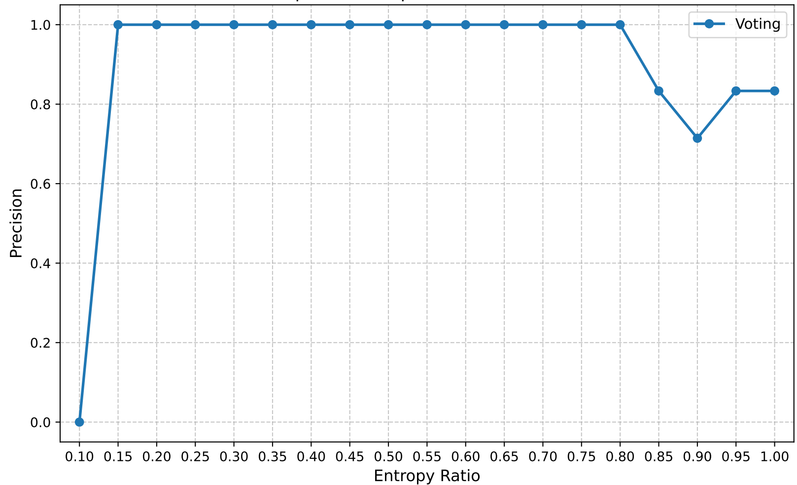
Precision | Round 25 | Confuse Model Ratio 0.50
