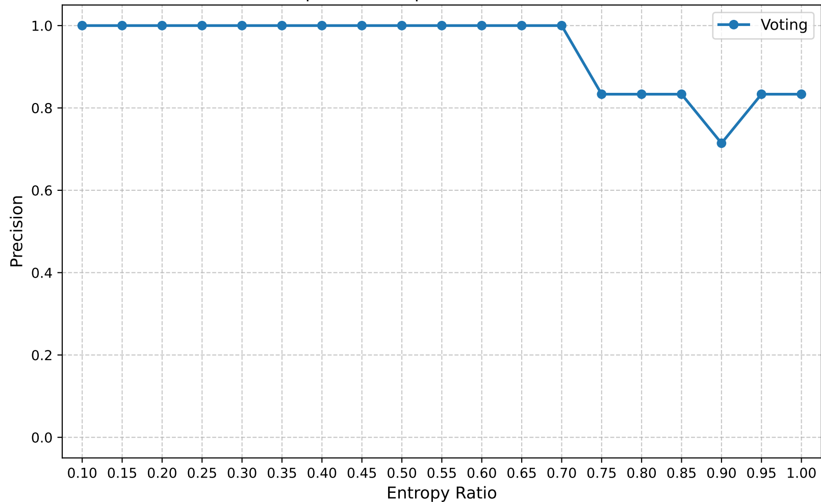
Precision | Round 25 | Confuse Model Ratio 0.60
