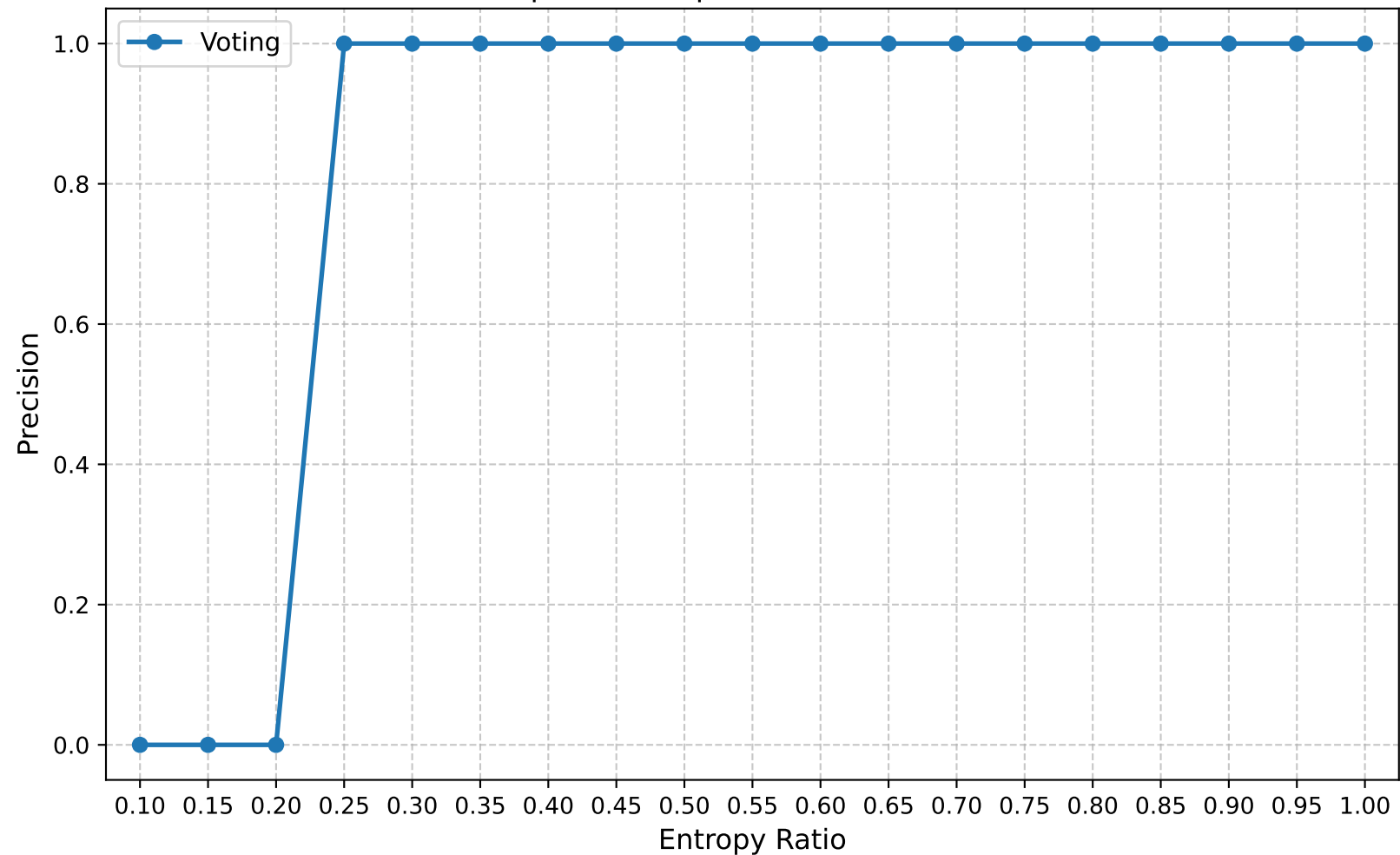
Precision | Round 5 | Confuse Model Ratio 0.10
