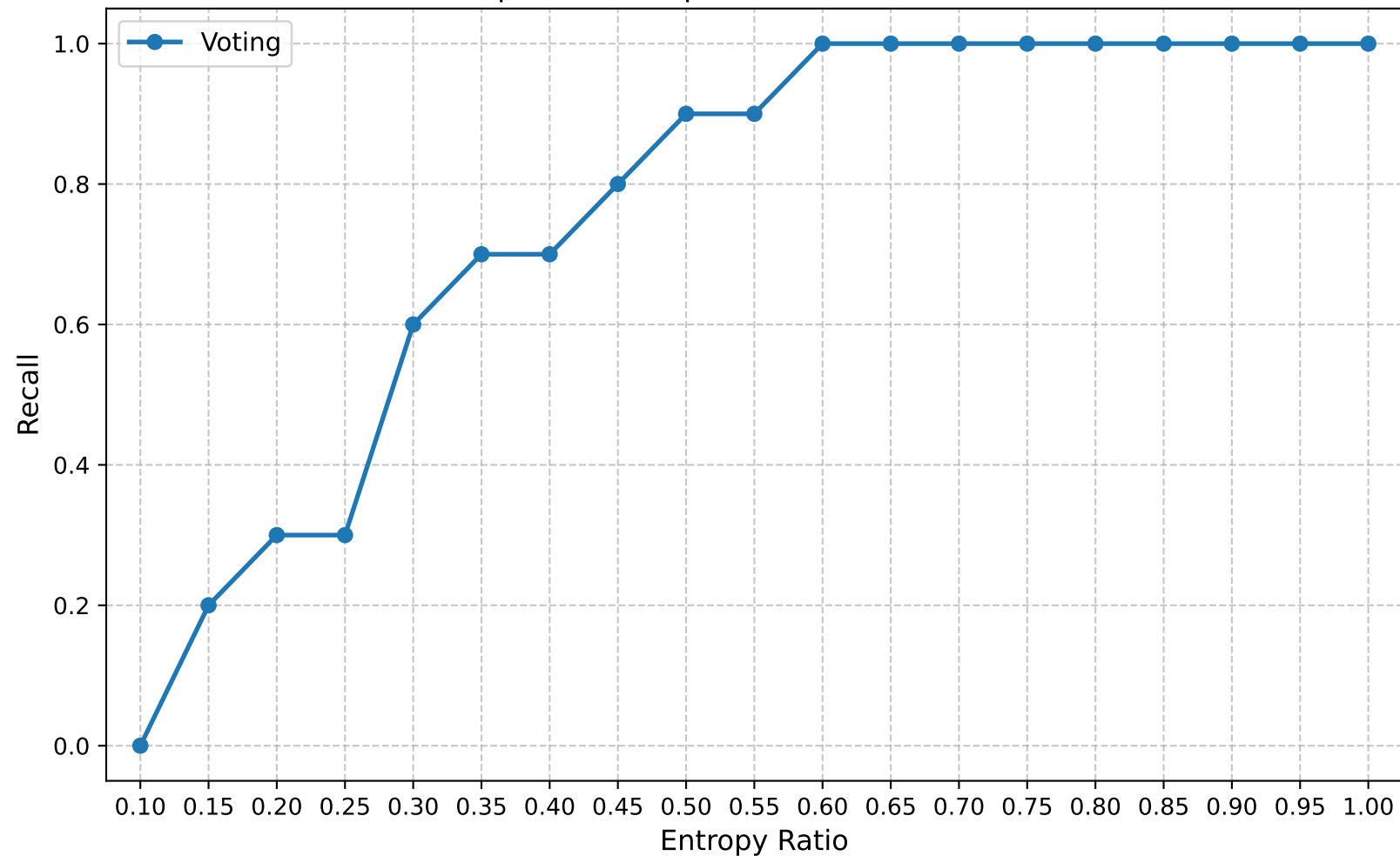
Recall | Round 10 | Confuse Model Ratio 0.50
