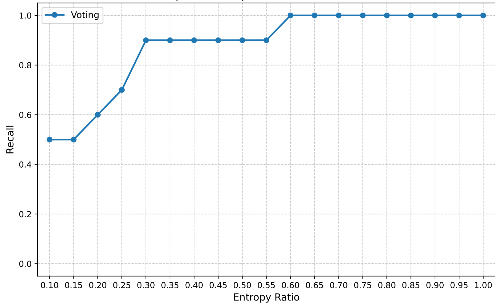
Recall | Round 10 | Confuse Model Ratio 0.90
