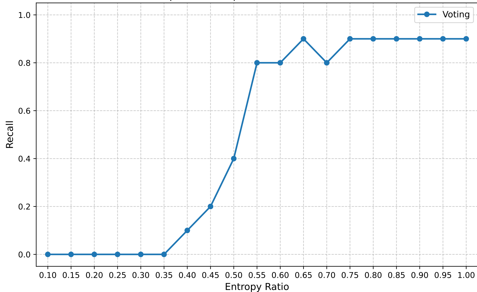
Recall | Round 15 | Confuse Model Ratio 0.10
