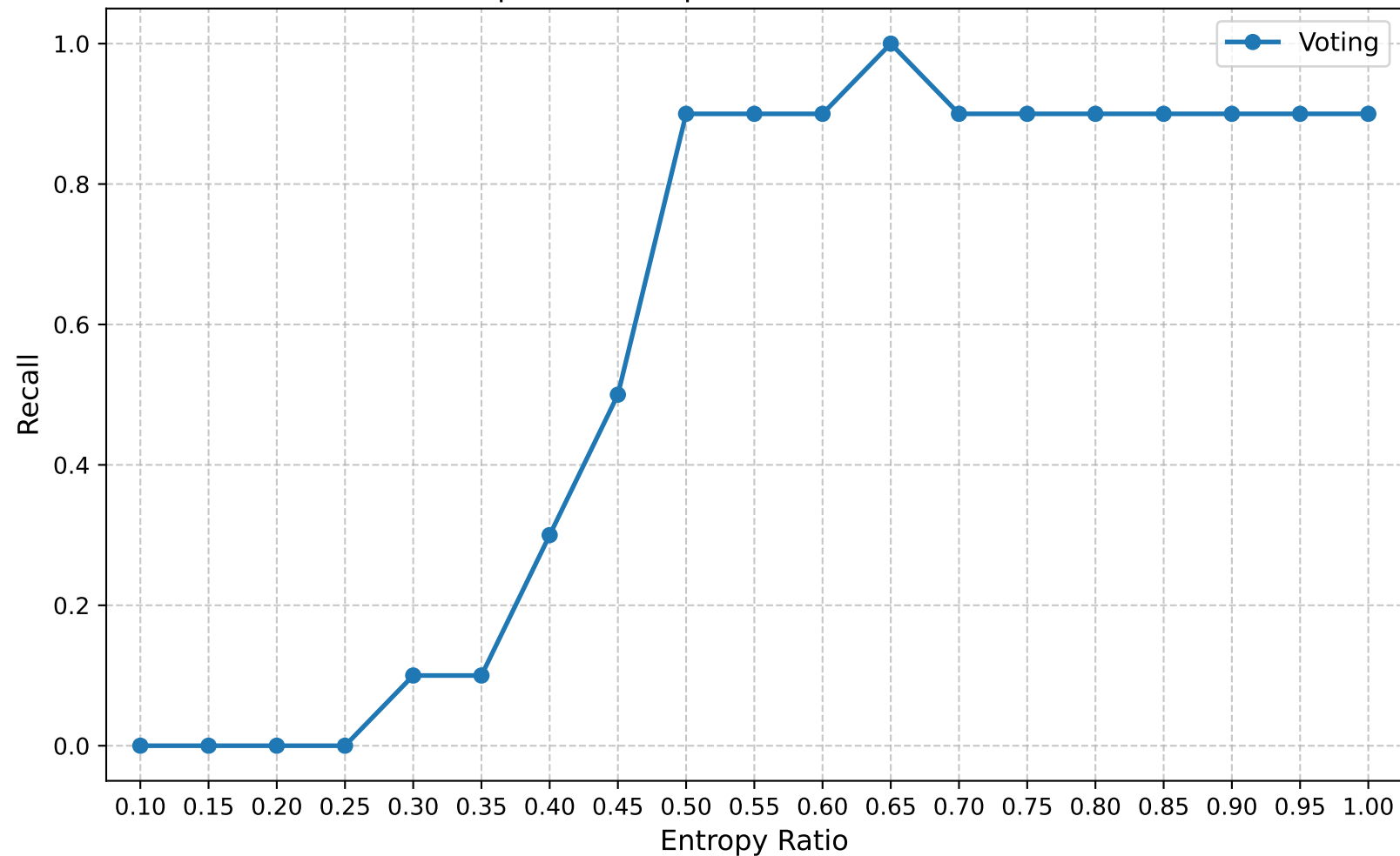
Recall | Round 15 | Confuse Model Ratio 0.20
